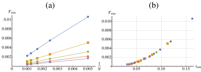
FIG. 3. (a) \mathcal{F}_{\min} as a function of N . Each line, from top- to bottommost, corresponds to an increasing value of \lambda \in (1.2, 2.0) in steps of 0.2. (b) Minimum value of \mathcal{F} vs corresponding required evolution time t_{\min} for different values of \lambda = 1.2 (circles), 1.4 (squares), 1.6 (diamonds), 1.8 (up triangles), 2.0 (down triangles). Each consecutive data point approaching the origin corresponds to an increasing value of N \in (200, 1000) in steps of 200.
