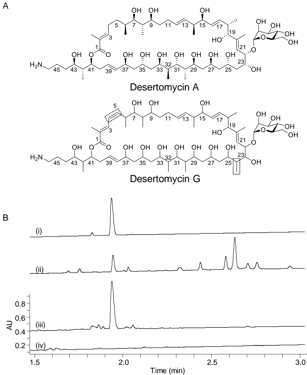
1 2 Figure 1. (A) Structure of desertomyicins A and G. The differences between the structures are shown by the 3 dotted rectangles. (B) HPLC chromatograms of authentic sample of desertomycin A (i), culture extracts 4 from S. nobilis JCM4274 (ii) and S. lividans TK23 carrying pKU518JCM4274_P1_P1-M4 (iii) and S. 5 lividans TK23 (iv). Chromatograms were traced at 220 nm.
