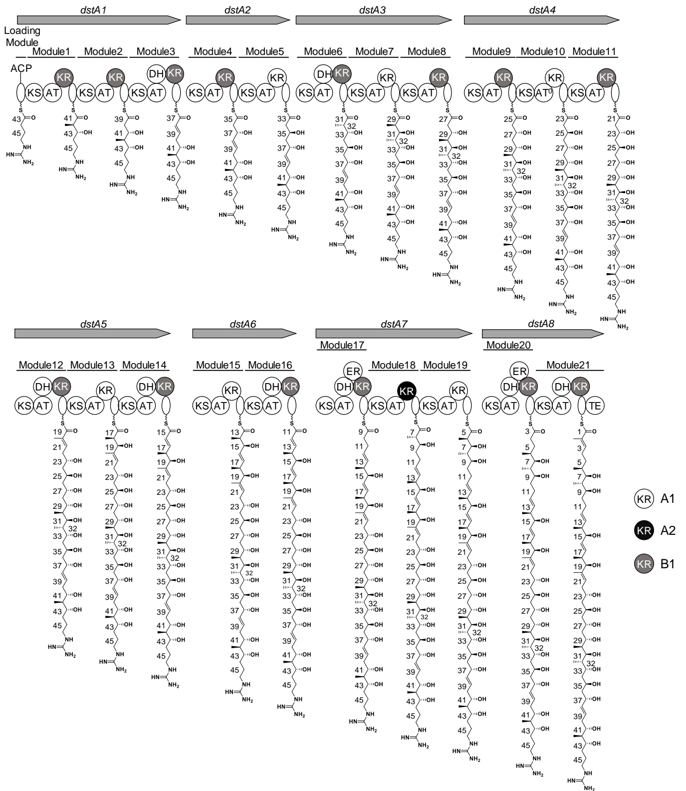
Figure 2. Proposed biosynthetic pathway by polyketide synthases encoded in dstA1-A8 .
