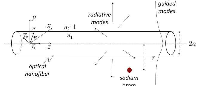
Figure 1. Sodium atom in the vicinity of an optical nanofibre with a radius a . The refractive index is n_1 = 1.45 for silica and n_2 = 1 for vacuum. The axis of the nanofibre is arbitrarily chosen as the z -axis. The cylindrical coordinates (r, \varphi, z) and frame (\vec{e}_r, \vec{e}_\varphi, \vec{e}_z) are introduced.
