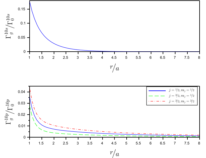
Figure 2. Spontaneous emission rate of a sodium atom into the guided modes of a nanofibre of radius a = 100 nm. The rate is plotted as a function of the distance r of the atom to the fibre axis: (top) atom initially prepared in the state |10s_{1/2}, m_j = \pm \frac{1}{2}\rangle , (bottom) atom initially prepared in the states |10p_{1/2}, m_j = \pm \frac{1}{2}\rangle , |10p_{3/2}, m_j = \pm \frac{1}{2}\rangle and |10p_{3/2}, m_j = \pm \frac{3}{2}\rangle . The rates \Gamma_g^{10s} , \Gamma_g^{10p} are presented relative to the spontaneous emission rates \Gamma_0^{10s} , \Gamma_0^{10p} in vacuum.
