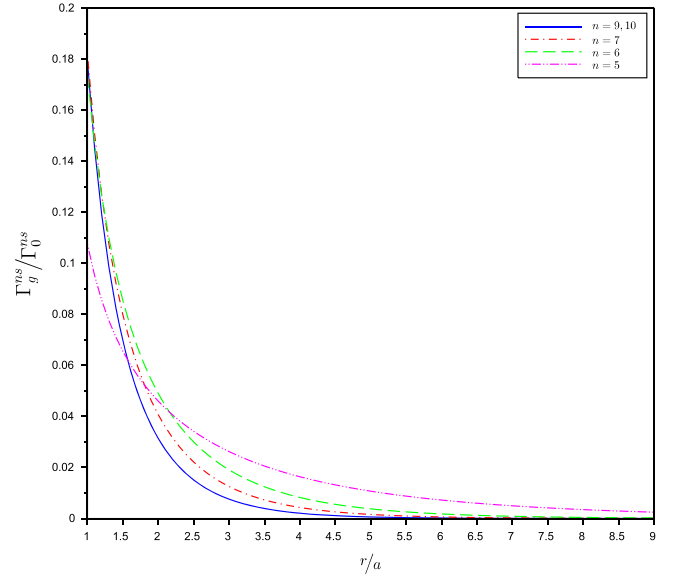
Figure 3. Spontaneous emission rate of a sodium atom initially prepared in |ns_{1/2}, m_j = \pm\frac{1}{2}\rangle , for n = 5, \dots, 10 , into the guided modes of a nanofibre of radius a = 100 \text{ nm} . The rate is plotted as a function of the distance r of the atom from the fibre axis. The rate, \Gamma_g^{ns} , is renormalized by the spontaneous emission rate in vacuum, \Gamma_0^{ns} , and the distance r is expressed in units of the fibre radius, a .
