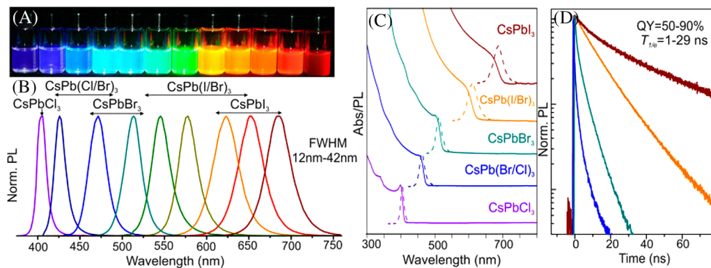
FIGURE 7 A, Photograph of colloidal \text{CsPbX}_3 NCs ( X = \text{Cl}, \text{Br}, \text{I} ) perovskite NCs in toluene under UV illumination. B, PL spectra exhibiting composition-tunable bandgap energies covering the entire visible spectral region with narrow and bright emission. C, Absorption and PL spectra corresponding to optical absorption and emission spectra of colloidal \text{CsPbX}_3 NCs. D, Time-resolved PL decays of colloidal \text{CsPbX}_3 perovskite NCs. Reproduced with permission. 64 Copyright 2015, American Chemical Society. NCs, nanocrystals; PL, photoluminescence
