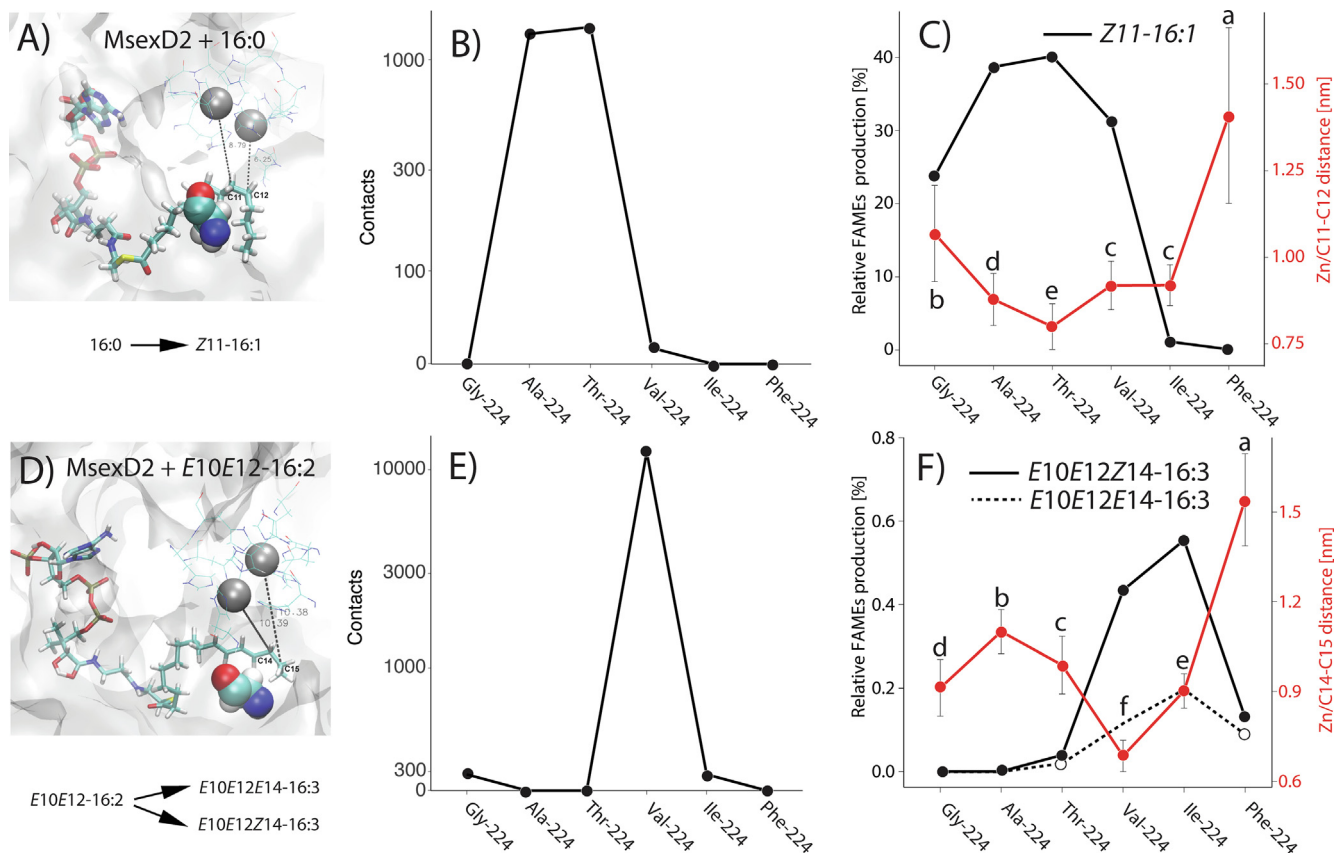
Fig. 4. Molecular dynamics simulations of MsexD2 with 16:0-CoA (A, B, C) and E10E12-16:2 -CoA (D, E, F) substrates in the substrate-binding tunnel. Snapshots from MD simulations of MsexD2 with 16:0-CoA (A) and E10E12-16:2 -CoA (D) substrates show Ala224 in van der Waals representation; Zn atoms in the active site are shown in grey surrounded by His residues and water molecules. Atoms belonging to the single bond of the substrate where desaturation takes place are labeled, along with the corresponding distance to Zn atoms in the active site. The total number of contacts (less than 0.7 nm) between the Zn atoms in the enzyme active center and the C11–C12 atoms of 16:0-CoA (B) and the C14–C15 atoms of E10E12-16:2 -CoA (E) are indicated. The average distances \pm SD between Zn atoms and desaturated carbon atoms are plotted together with relative unsaturated fatty acyl production (C,F) reproduced from Fig. 3, with SD bars omitted for clarity. The average distances which are significantly different ( \alpha = 0.05 ) in ANOVA with “post-hoc” Tukey’s test are marked with different letters.
