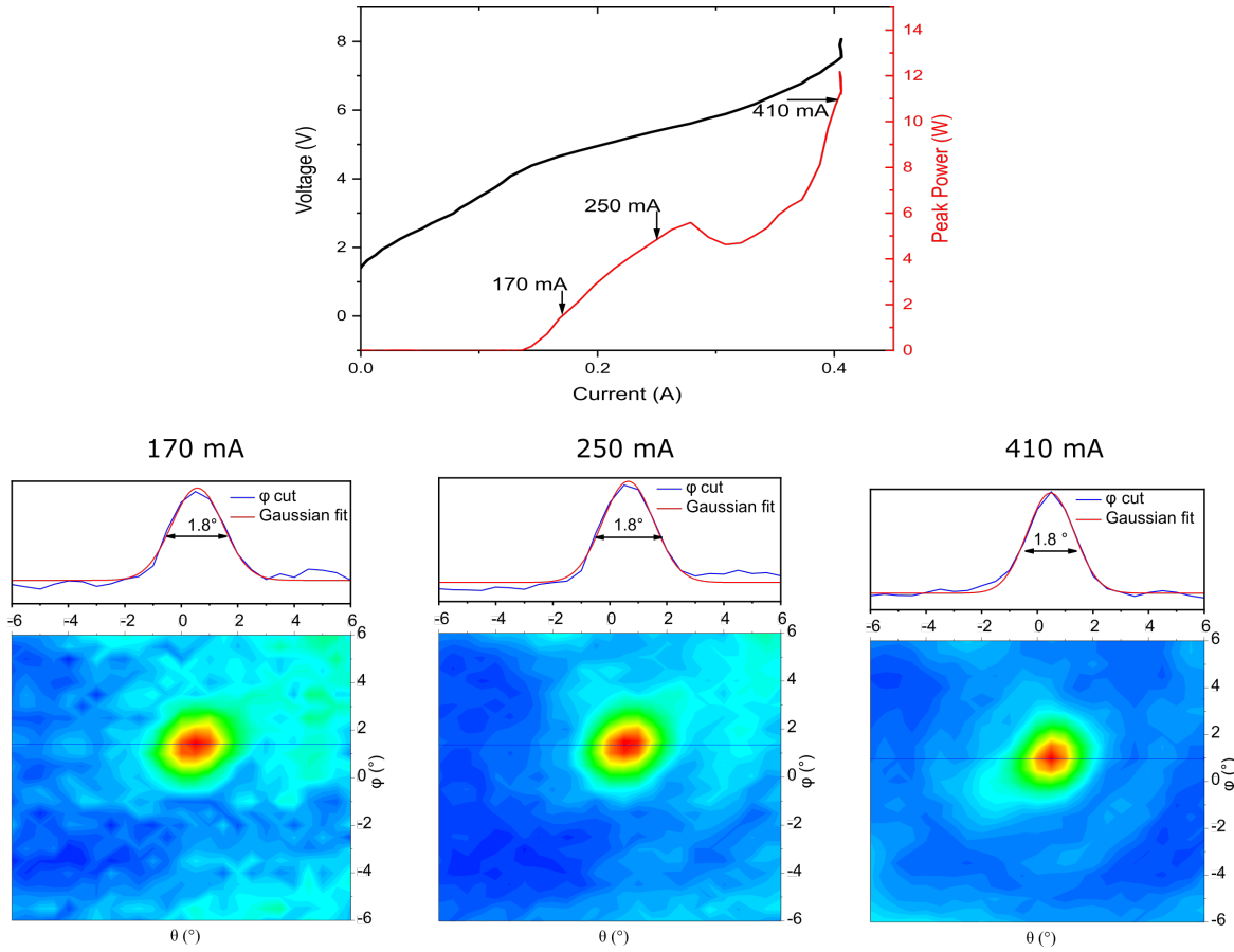
Figure 3.14: LIV curves and far-field intensity maps for sample s=15\text{ }\mu\text{m} , d=15\text{ }\mu\text{m} . Data taken for three different bias currents. Profile taken in the \phi direction. FWHM values calculated by fitting the \phi cut with a Gaussian fit.
