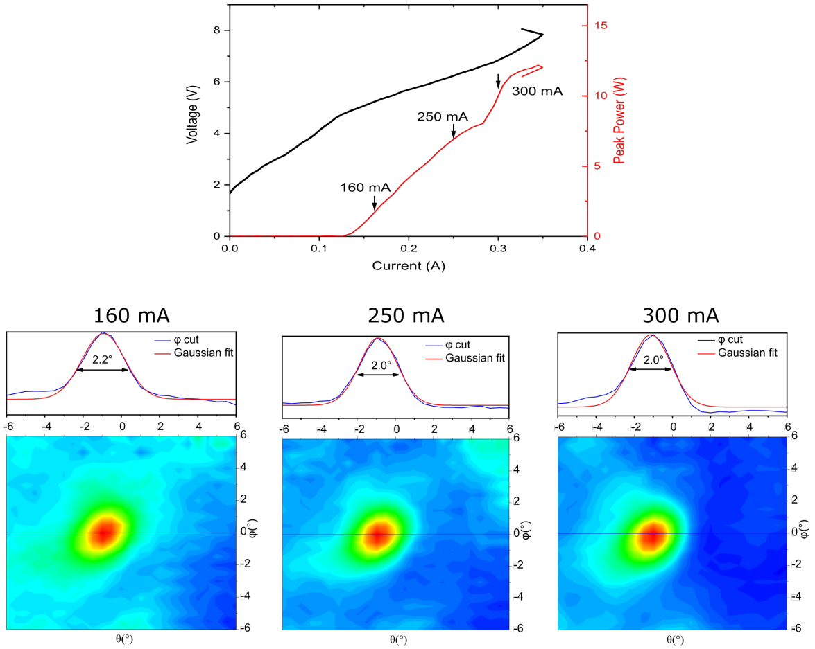
Figure 3.15: LIV curves and far-field intensity maps for sample s=15\text{ }\mu\text{m} , d=25\text{ }\mu\text{m} . Data taken for three different bias currents. Profile taken in the \phi direction. FWHM values calculated by fitting the \phi cut with a Gaussian fit.
