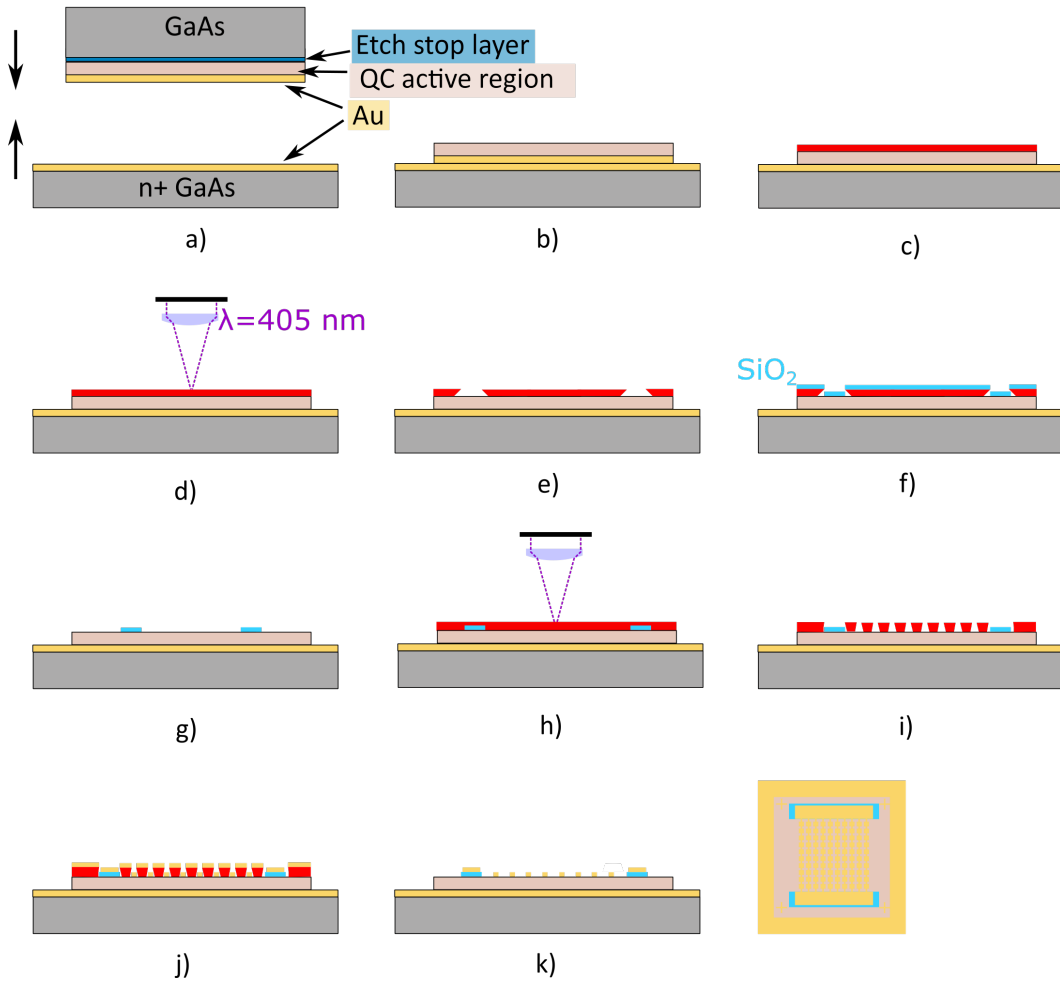
Figure A.1: Fabrication procedure. a) Wafer bonding. b) Substrate removal. c) Photoresist spin coating. d) 1st layer Photolithography. e) Development of photoresist. f) \text{SiO}_2 thin film sputtering. g) Lift-off. h) Lithography 2nd layer. i) Development of 2nd layer photoresist. j) Ti/Au thin film deposition. k) Lift-off. Process finishes.
