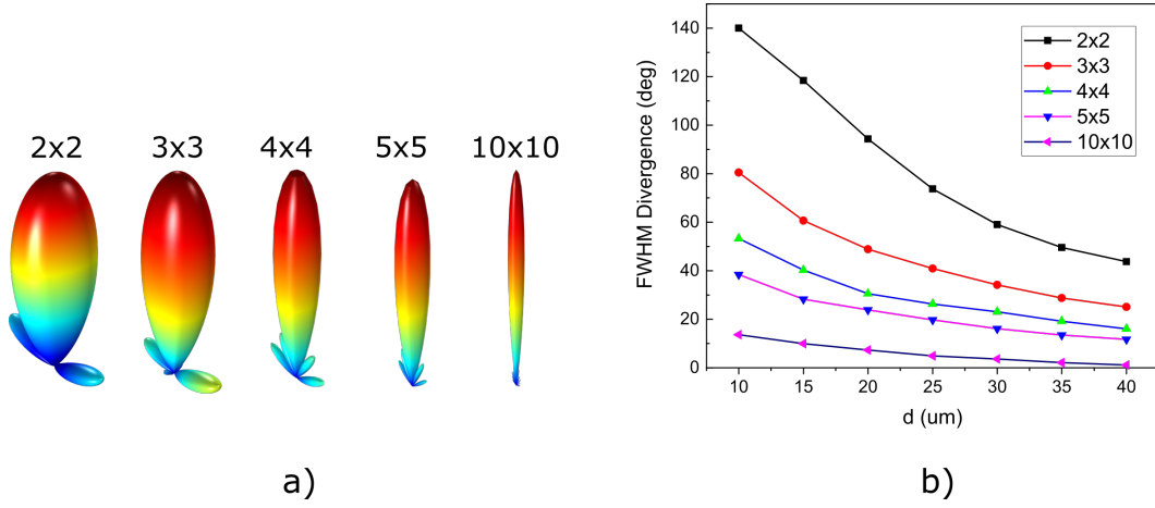
Figure 3.19: Far-field simulations for varying d and N . a) 3D far-field patterns emitted by N \times N planar arrays with N = 2, 3, 4, 5 and 10 . (Distance is fixed to d = 40 \mu\text{m} ). b) Calculated FWHM for different array configurations as a function of the distance of separation between elements d .
