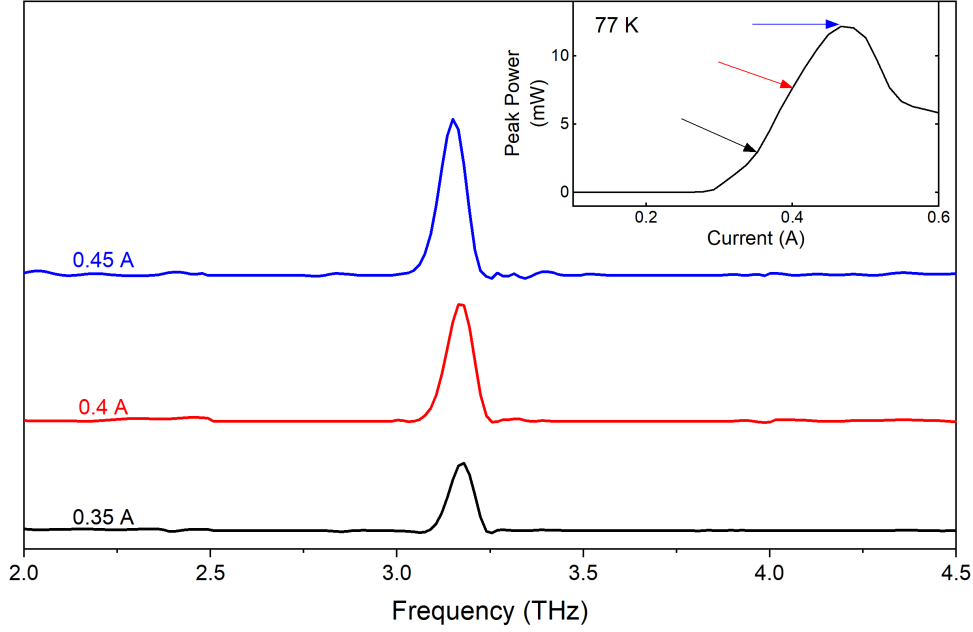
Figure 3.11: Spectra of a PAM THz QCL. Array parameters: s=15\ \mu\text{m} , d=40\ \mu\text{m} . Data taken at a heat sink temperature of 77 K for three different bias currents. Inset: Sample's L-I curve. Arrows indicate the intensities at which FTIR measurements were taken.
