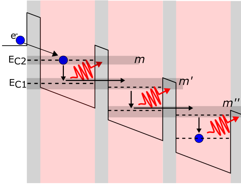
Figure 1.4: Schematic representation of the operating principle of a QCL. Red areas represent the quantum wells and gray areas the barriers. Arrows indicate the movement of electrons through the material. An electron is injected into the excited state E_{C2} contained in a miniband m (gray-shaded area) and undergoes optical transition by decaying to a lower energy state E_{C1} of a miniband m' . Photons are emitted in every stage (red curved arrow). After every emission, electrons tunnel to the next QW where another optical transition happens.
