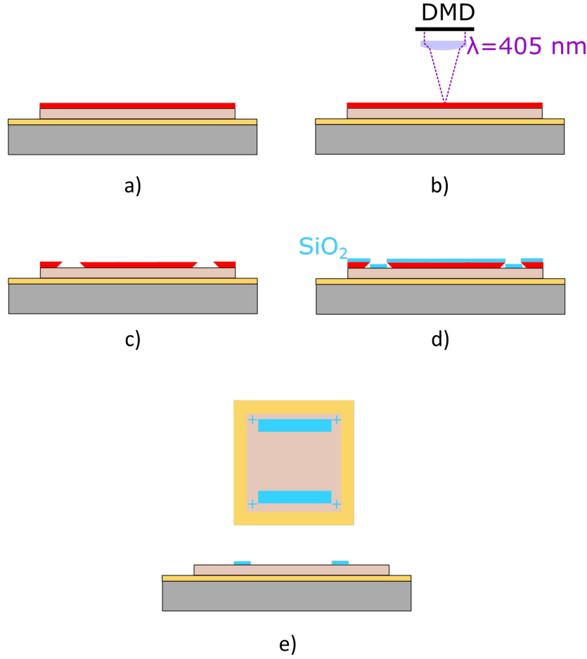
Figure 3.4: Photolithography for the 1st layer and SiO 2 deposition. a) A negative photoresist (ARN 4450) is spin-coated on the surface of the QC sample. b) Exposure of the resist using a maskless lithography system [NANO SYSTEM SOLUTIONS Dlight DL-1000]. c) Development of the photoresist, undercut profiles are achieved. d) A thin film of SiO 2 is sputtered on the sample's surface. e) Lift-off. Insulating pads and reference marks are created on top of the QC sample.
