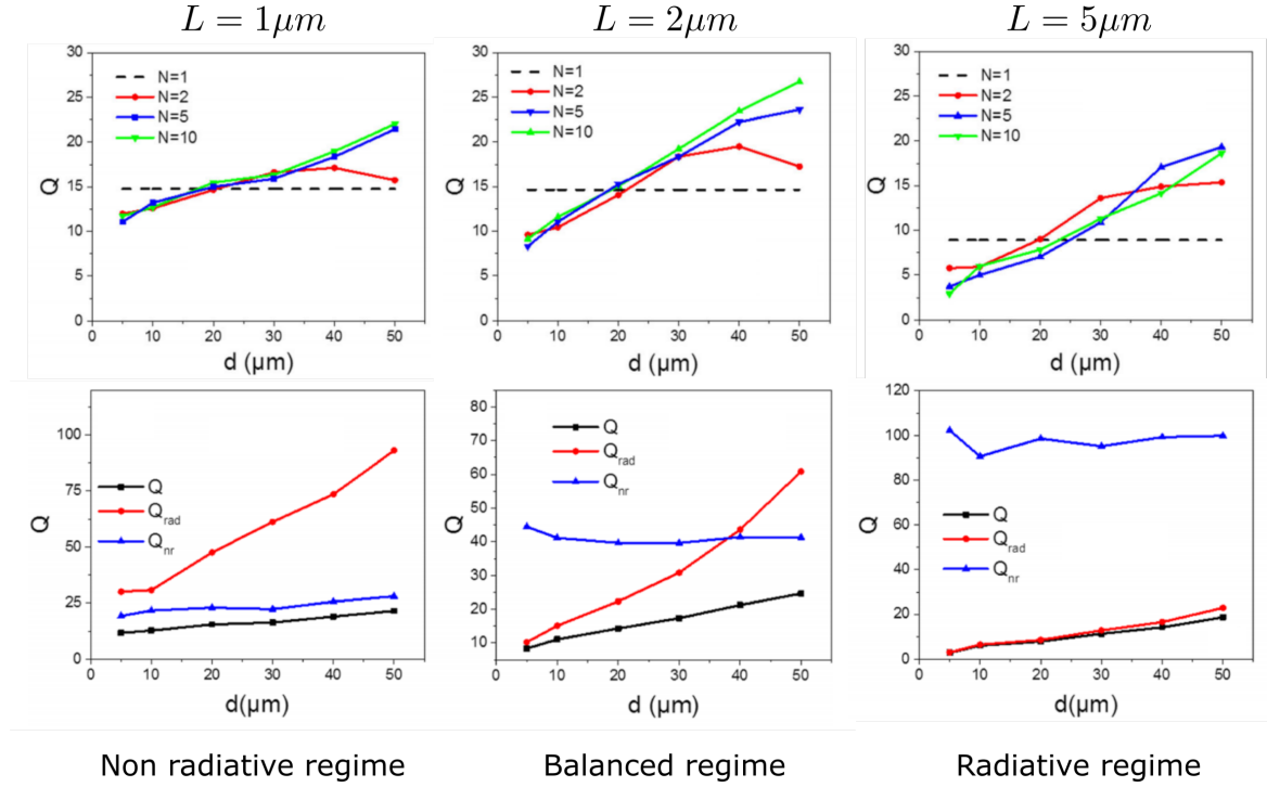
Figure 2.9: Quality factors vs distance between resonators. First row: quality factors of the system as a function of the separation distance d between resonators for various N . Second row: comparison between total, radiative and non-radiative quality factors vs d for an array with N = 10 elements. Plots taken from [118] .
