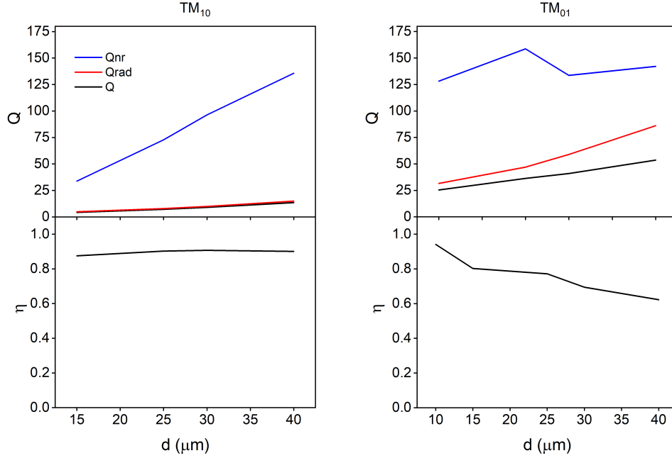
Figure 2.16: Comparison between total, radiative, and non-radiative quality factors vs distance d in wired arrays and extraction efficiencies. Comparison between the TM 10 and TM 01 modes for s = 16 \mu\text{m} .
