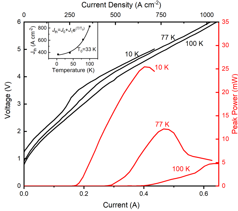
Figure 3.9: LIV data for a PAM array. Array parameters: s=15\ \mu\text{m} , d=40\ \mu\text{m} . Data taken for three different operating temperatures: 10 K, 77 K and 100 K. Black curves represent the voltage-current data, while red curves the power-current data. Inset: threshold current density as a function of the heat sink temperature (fit based on the empirical formula J_{th} = J_0 + J_1 e^{T/T_0} ). Adapted from [126].
