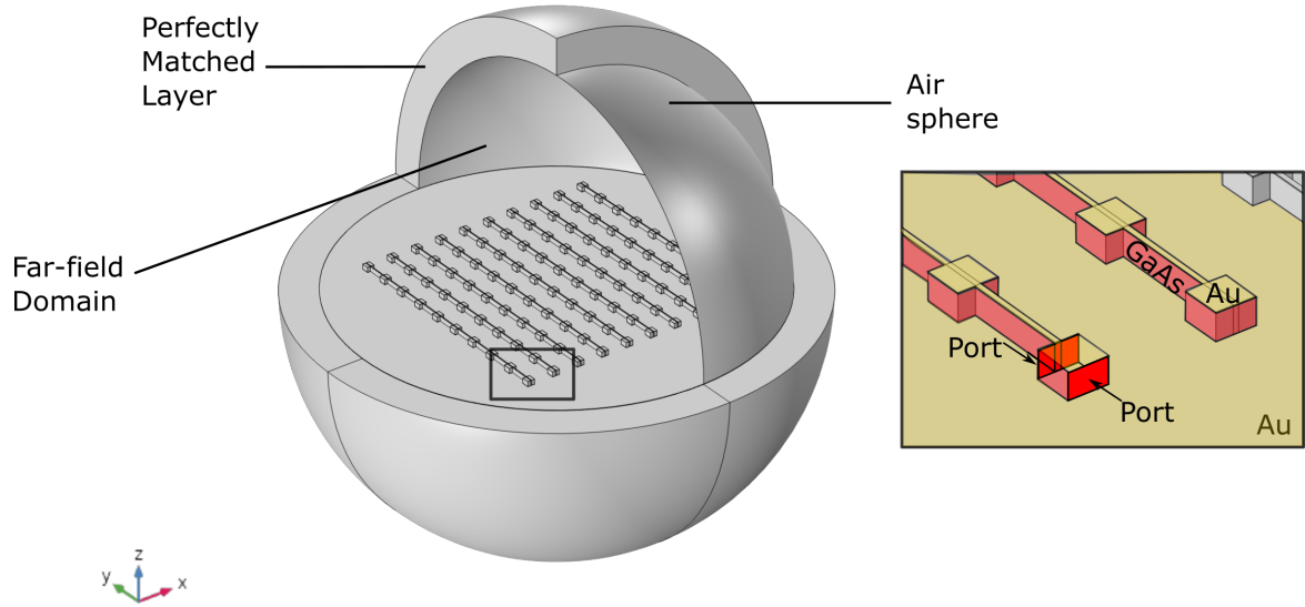
Figure 3.17: 3D simulation model. Model consists a wired patch antenna micro-cavity array enclosed by an air sphere domain bounded by a perfectly matched layer. Black rectangle contains a close-up view of a section of the array.
