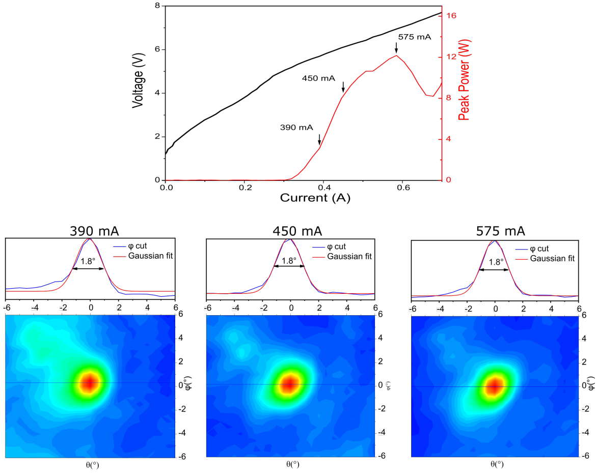
Figure 3.16: LIV curves and far-field intensity maps for sample s=15\ \mu\text{m} , d=40\ \mu\text{m} . Data taken for three different bias currents. Profile taken in the \phi direction. FWHM values calculated by fitting the \phi cut with a Gaussian fit.
