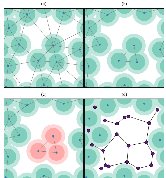
Fig. 5. Illustration of the film portion filtering (FPF) algorithm: (a) Delaunay network formed from grain centers with r < r_m . (b) Network with edges larger than 2r filtered. (c) All network components, except the component consisting of most vertices, are marked to be treated as special pore components. (d) Pores after FPF together with the vertices and edges obtained with Algorithm 2 .
