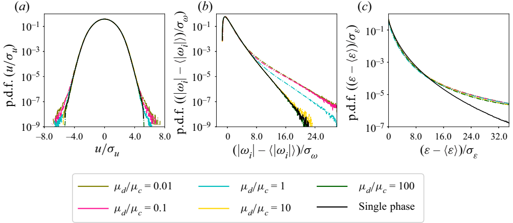
Figure 29. P.d.f.s of (a) velocity fluctuations u , (b) vorticity \omega , and (c) energy dissipation. All quantities are normalized by their standard deviations. The data pertain to cases V2x, with \alpha = 0.03 .
