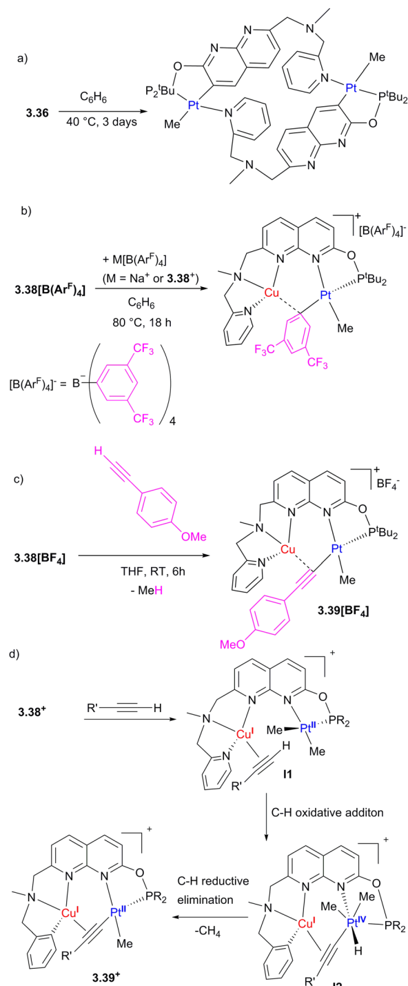
Scheme 31 Reactivity of Pt/Cu complexes: (a) rollover cyclometallation of a monometallic 3.36. (b) Aryl group transfer from the [B(Ar F ) 4 ] - (B(Ar F ) 4 = tetrakis[3,5-bis(trifluoromethyl)phenyl]borate) to 3.38 + . (c) Reactivity of 3.38 + with a terminal alkyne. (d) Proposed mechanism of alkyne activation by 3.38 + .
