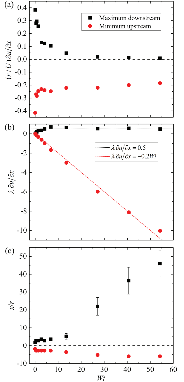
Figure 7: a) Value of the velocity gradient (non-dimensionalized by r/U ) measured at the downstream maximum and the upstream minimum and (b) the same velocity gradient non-dimensionalized by \lambda . (c) Non-dimensionalized x -location of the downstream maximum and the upstream minimum velocity gradient as a function of the imposed Weissenberg number.
