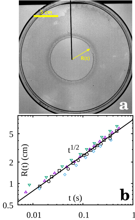
Figure 2: (a) Visualization of camphoric acid spread radius. The water surface is uniformly covered with 50 \mu\text{m} hollow glass spheres at low packing fractions to visualize the spread dynamics. Scale bar: 5 cm (b) Spread radius vs. time follows a t^{1/2} scaling law. Different symbols indicate different trials.
