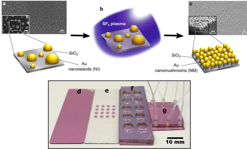
Figure 1: Transforming Au Nanoisland (NI) precursors to nanomushroom (NM) arrays in \text{SF}_6 plasma: a) Scanning electron microscopy (SEM) image (Quanta 250 FEG, 5 KV, 100 kX magnification) and schematic of NIs. b) Schematic showing a \text{SiO}_2 substrate with NIs inside a \text{SF}_6 plasma chamber, where \text{SF}_x reactive ions etch out both \text{SiO}_2 and Au. c) SEM image and schematic of NMs formed after exposure to reactive ion etching inside \text{SF}_6 plasma. The inset shows the cross section of the NMs. The developed NM structures are 45–60 nm in total height with an average spacing of 7.96 \pm 2.12 nm. Examples of various configurations of NM substrates or integrated chips: d) NM coated glass slide of size 2.5 cm \times 7.5 cm. The pink color corresponds to the Au nanostructures; e) Spots of 3 mm circles for multiplex bioassay applications; f) Integrating PDMS wells on a NM substrate; g) Sealed device with PDMS microfluidic channels on a NM substrate, connected with liquid delivery tubings.
