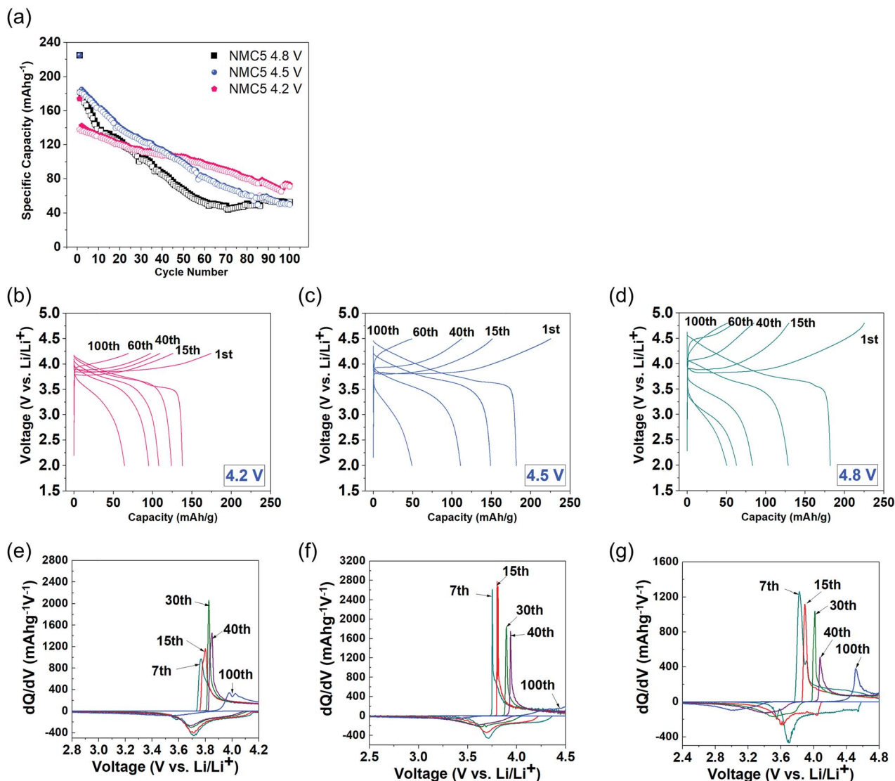
Fig. 1 Electrochemical properties of Li(Ni 0.5 Mn 0.3 Co 0.2 )O 2 (NMC5) cells at different cut-off voltage levels: (a) comparison of charge and discharge capacities for 100 cycles and the galvanostatic profiles at (b) 4.2 V cut-off voltage, (c) 4.5 V cut-off voltage, and (d) 4.8 V cut-off voltage with 0.4 C-rate current applied. The corresponding dQ/dV plots of (e) 4.2 V, (f) 4.5 V, and (g) 4.8 V cut-off voltages for the 7th, 15th, 30th, 40th, and 100th cycles.
